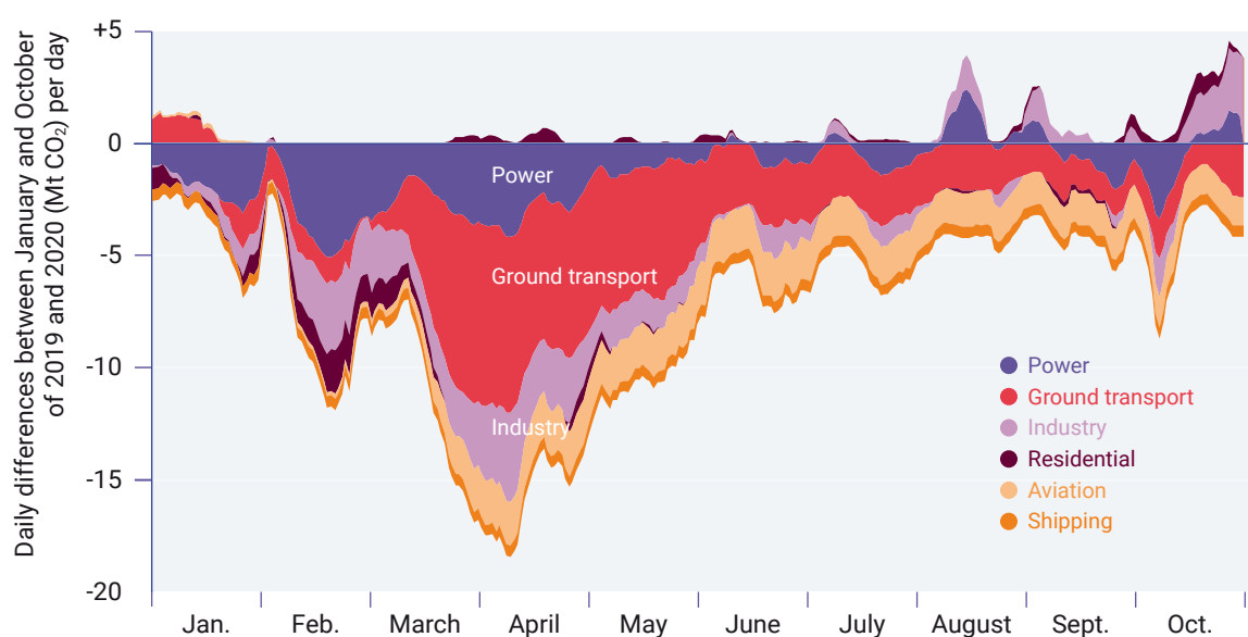
Figure ES.3. Reduction in emissions in 2020 relative to 2019 levels due to COVID-19 lockdowns
